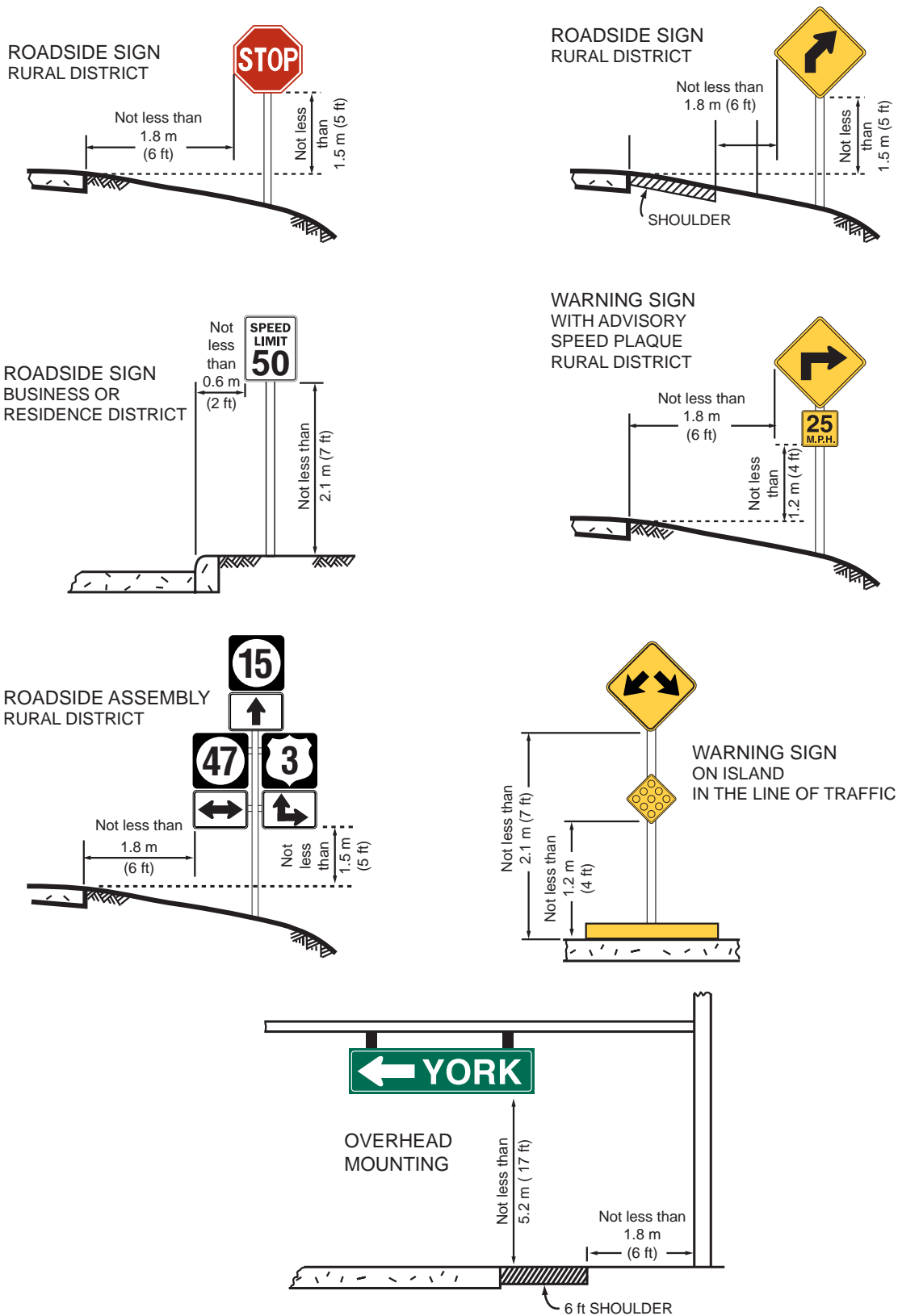
Figure 2A-1. Height and Lateral Location of Signs for Typical Installations
